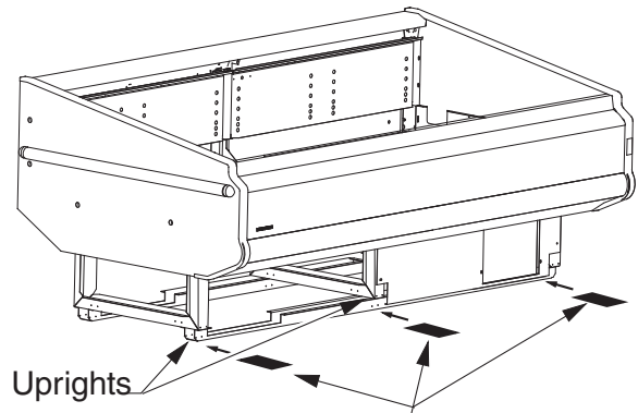
Install Shims under Rails at Uprights Only
