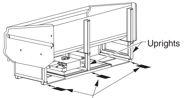
Install Shims under Rails at Uprights Only
