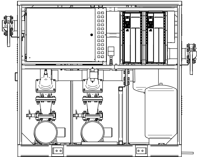
FRONT VIEW WITHOUT DOORS ARMSTRONG PUMPS CONFIGURATION SHOWN, B & G IS DIFFERENT
