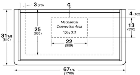
IM-X-E5-H End Module
