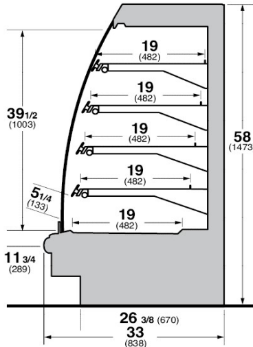
IM-X-E5-H End Module
