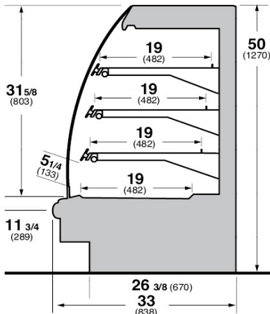
IM-X-C5-H Center Module / IM-X-I5-H Q-Series Match
