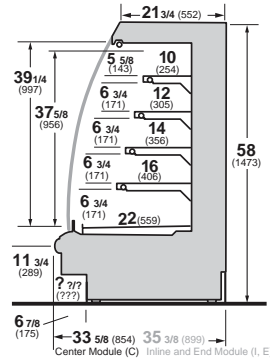
IM-X-05-R Refrigerated Self-Service Module
