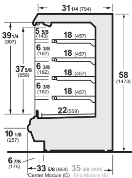
IM-X-05-R-EC10 Refrigerated Self-Service Module
