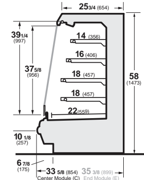
IM-X-05-R-EC Refrigerated Self-Service Module
