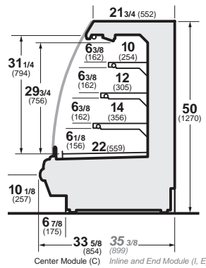
IM-X-04-R Refrigerated Self-Service Module
